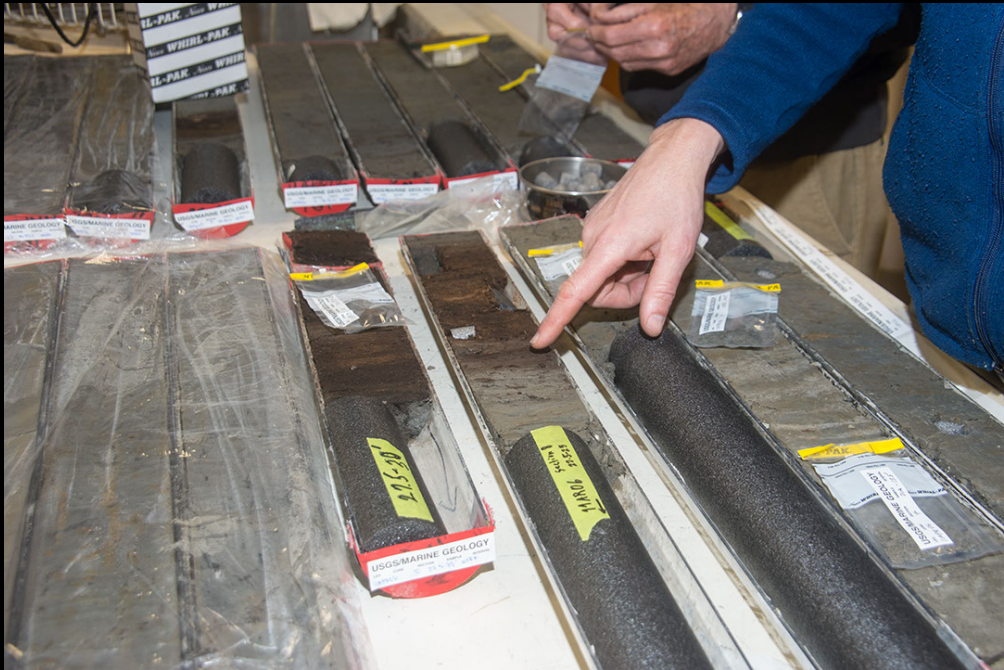
131205-0392_Peat_compressed
