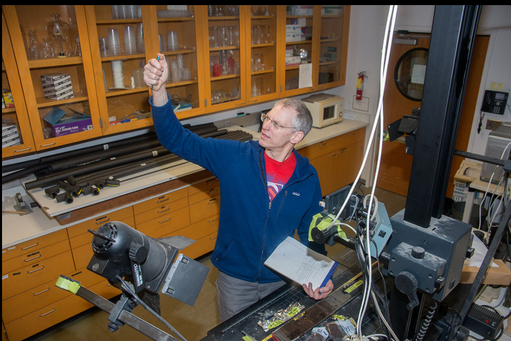
131205-0384_Platker_Haeussler_drill-core
